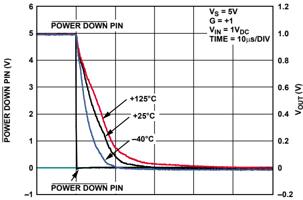
Figure 30. POWER DOWN Time vs. Temperature
