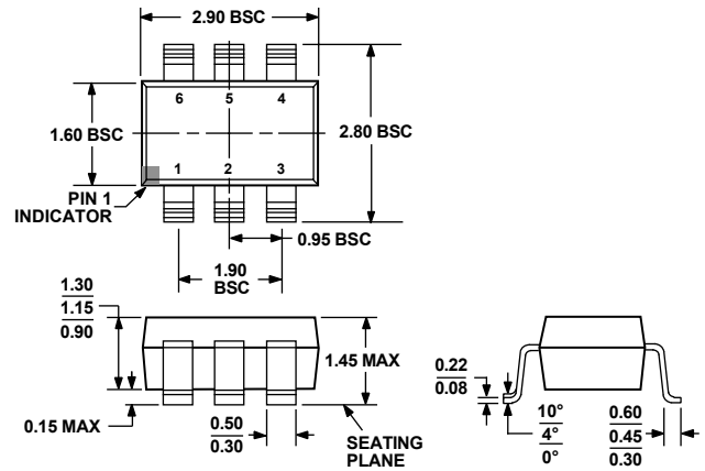
Figure 54. 6-Lead Small Outline Transistor Package [SOT-23] (RJ-6)
