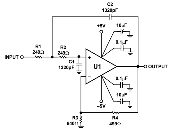
Figure 50. Two-Pole 500 kHz Reconstruction Filter Schematic
