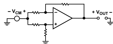
Figure 44. Common-Range Subtractor
