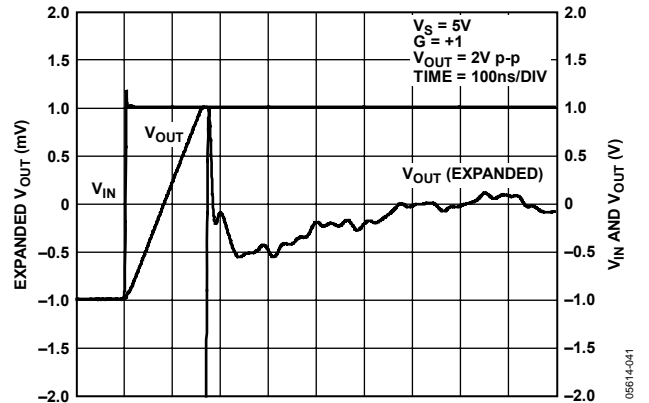
Figure 28. Settling Time
