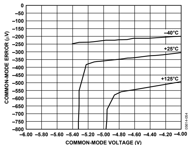
Figure 43. -CMV vs. Common-Mode Error vs. V_{OS}
